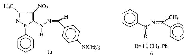
Figure 2. Structure of compounds 1a and 6 .
