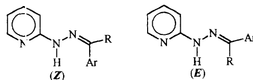
Figure 6. (E) and (Z) diastereomers for derivatives 5 .
