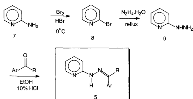
Figure 5. Synthesis of 2-pyridylhydrazone derivatives.
