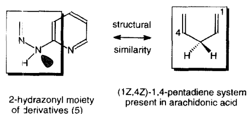
Figure 3. Structural relationship between the (1Z,4Z)-1,4-pentadiene system of arachidonic acid and the 2-pyridyl-arylhydrazone derivatives 5 .
