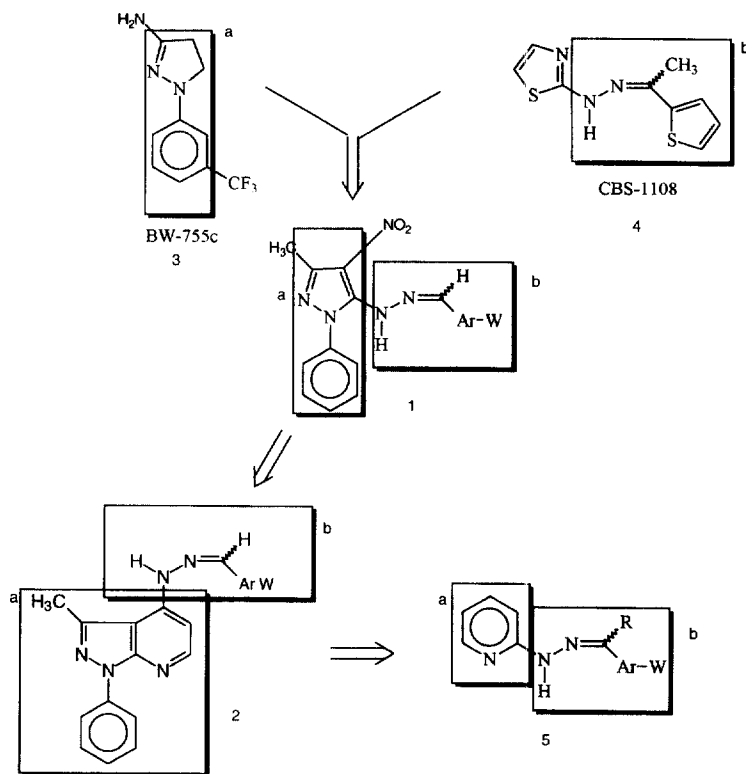
Figure 1. Genesis of 2-pyridylarylhydrazone derivatives 5 .
