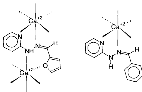
Figure 7. Representation of chelating \text{Ca}^{2+} for derivatives 5d (W = H) and 5p (Ar = 2-furyl).
