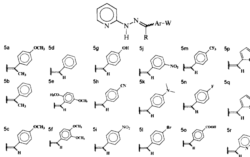
Figure 4. New 2-pyridylarylhydrazone derivatives 5a-r .
